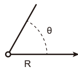
Fig. 3. A polar coordinate system
